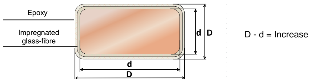
Conductor tolerances
