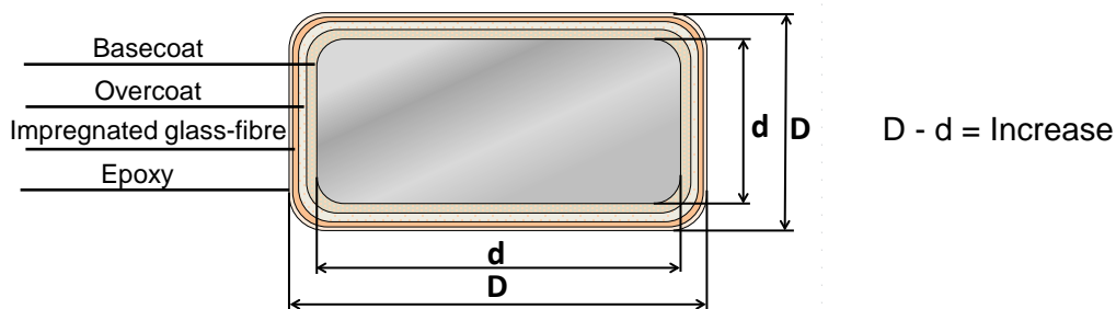
Conductor tolerances
